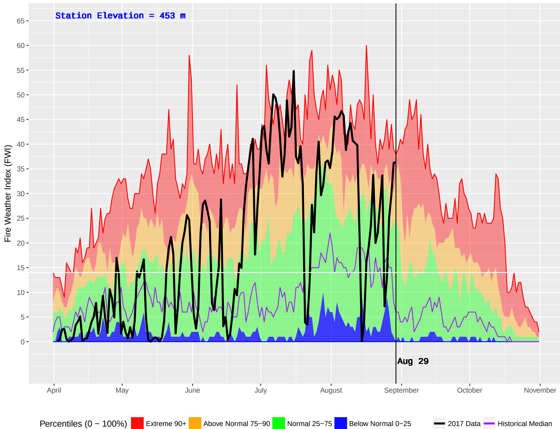
CLEARWATER HUB (239) : Historical (1976–2016) and Current (2017) Noon Fire Weather Index (FWI)
